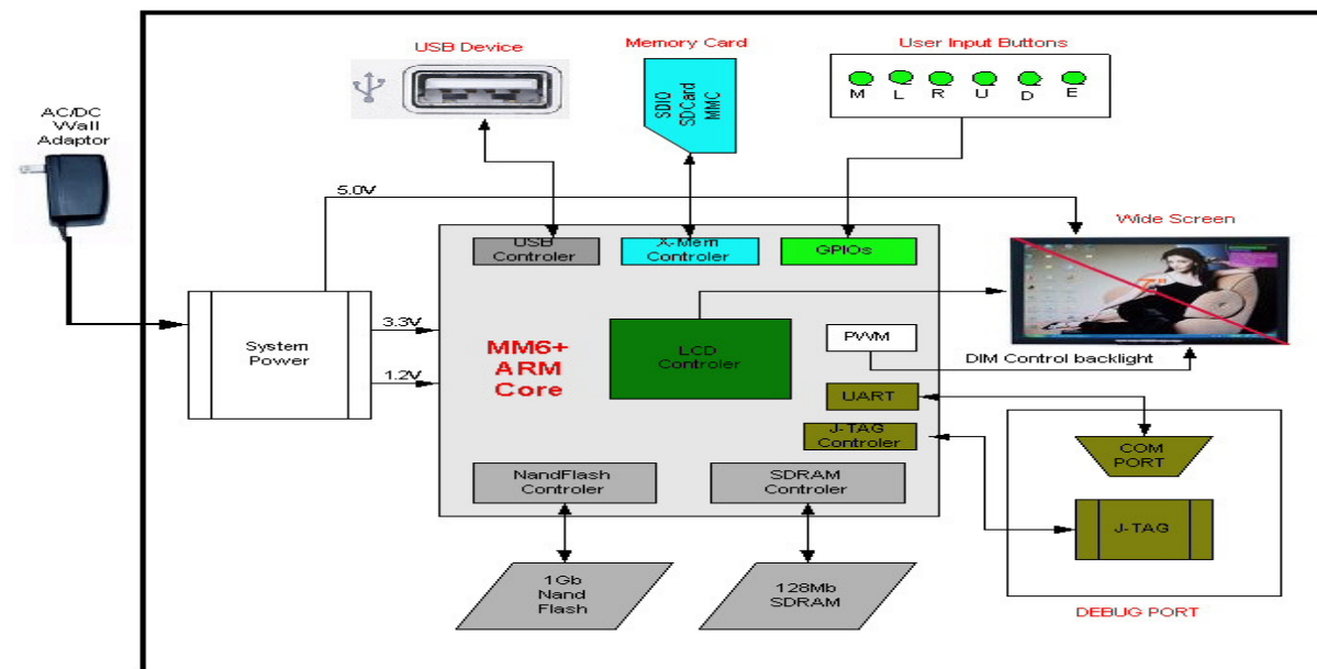
DIGITAL PICTURE FRAME BLOCK DIAGRAM
